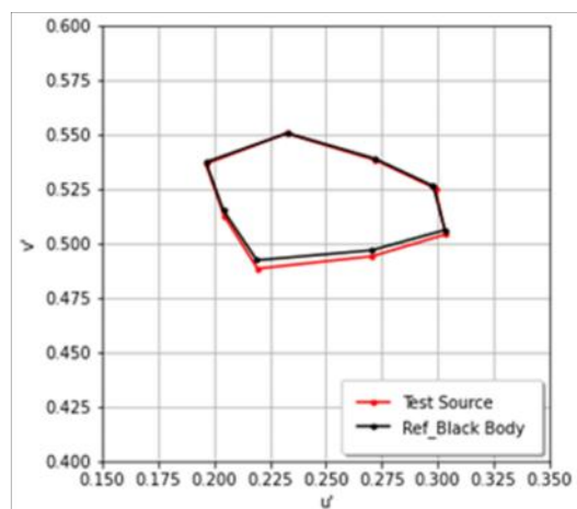
Gamut Area Reference to Black Body Radiator (8 TCS Samples)
