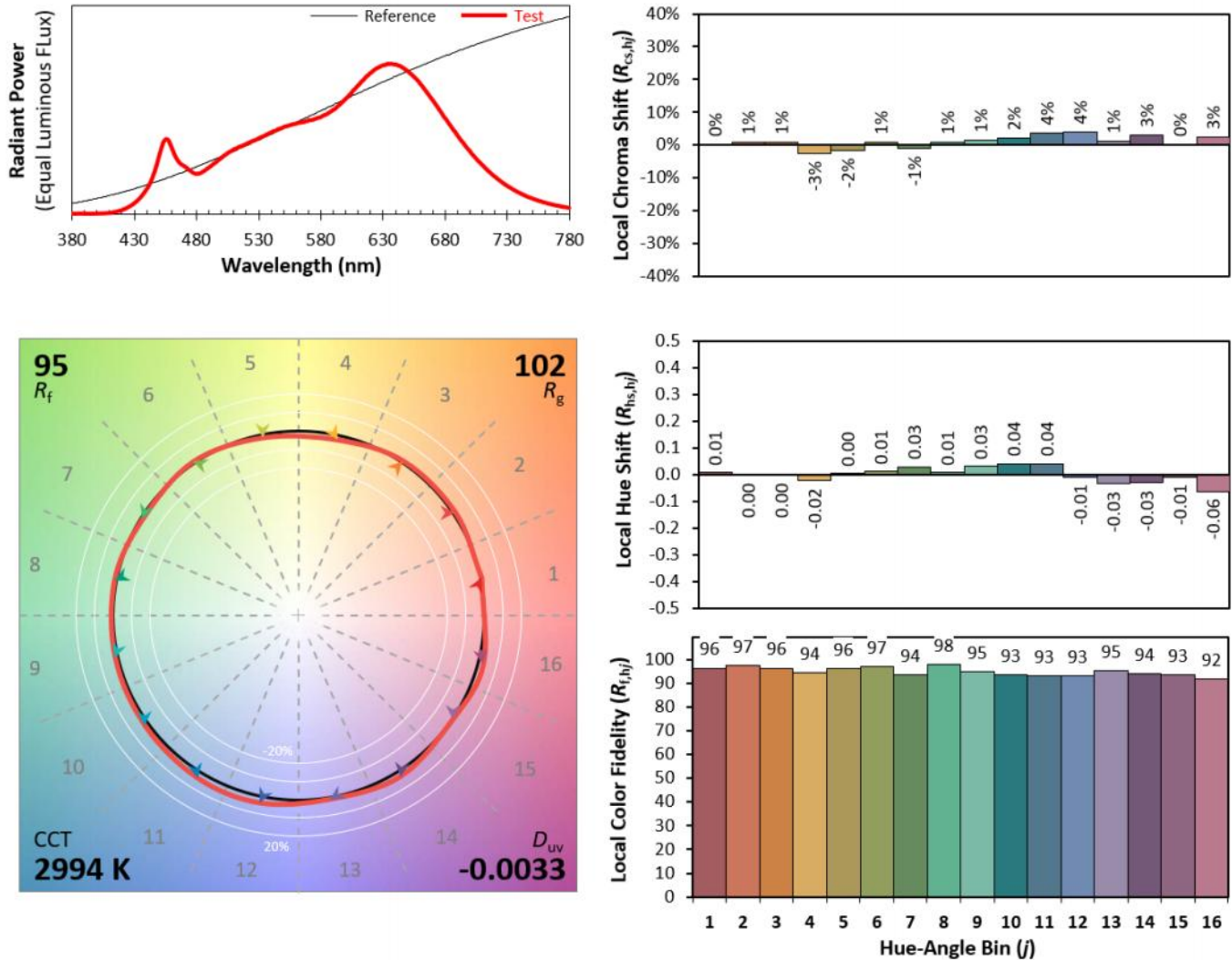
Figure 30 - The TM-30-18 report for Luminus COB Hospitality Series LEDs (30-95-TC41), demonstrating excellent color rendition performance with close match of the circles in the color vector graphic and average of Hue-Angle bins show color fidelity ( R_f ) of 95 [P1, V3, F1].
